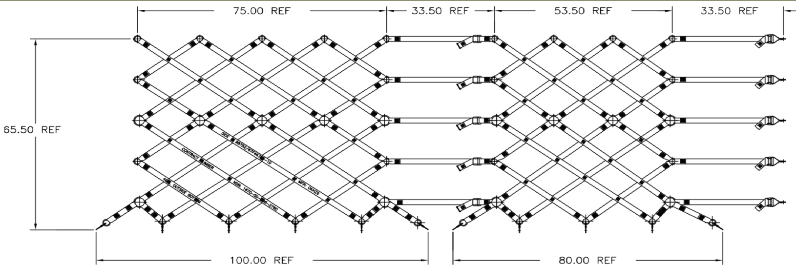
Kinedyne HCU-7/E Side Cargo Net
